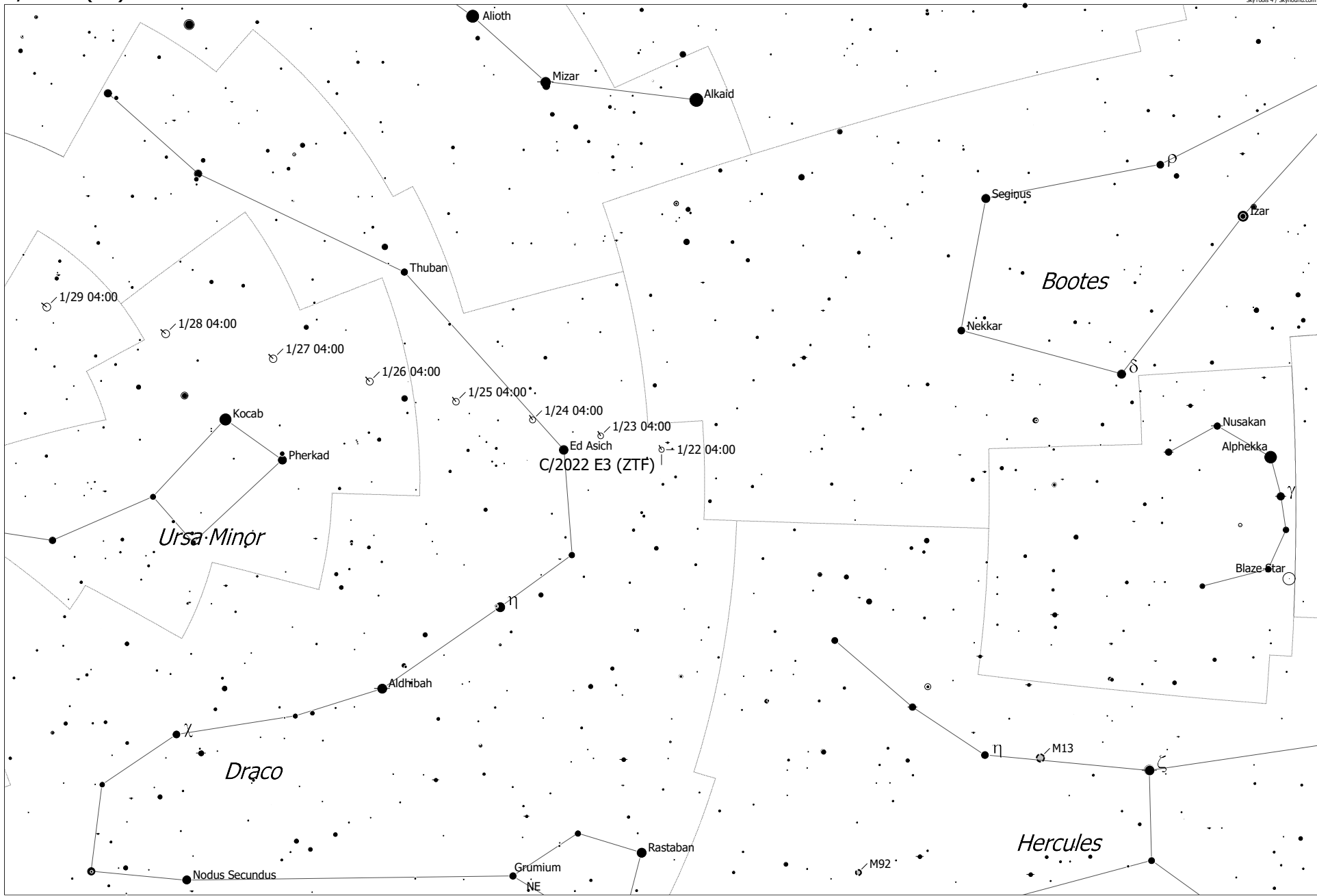
2023 January 22 04:00, East Point Fully dark (optimum conditions) C/2022 E3 (ZTF) (Comet) Magnitude: 5.94 Coma Diameter: 15.5' SBR: 20.5 Mag/arcsec 2 Earth Distance: 0.4 AU
